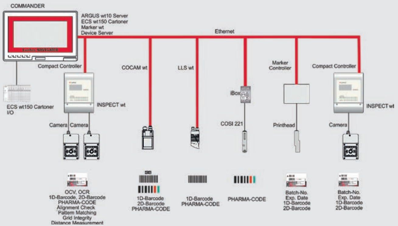
ARGUS WT SYSTEM ARCHITECTURE
